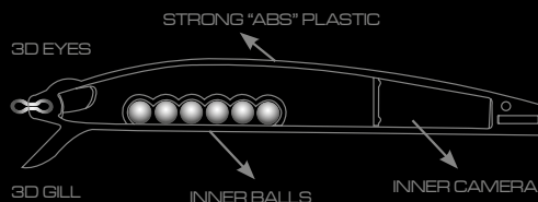
INSIDE VIEW
