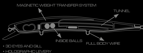
INSIDE VIEW
